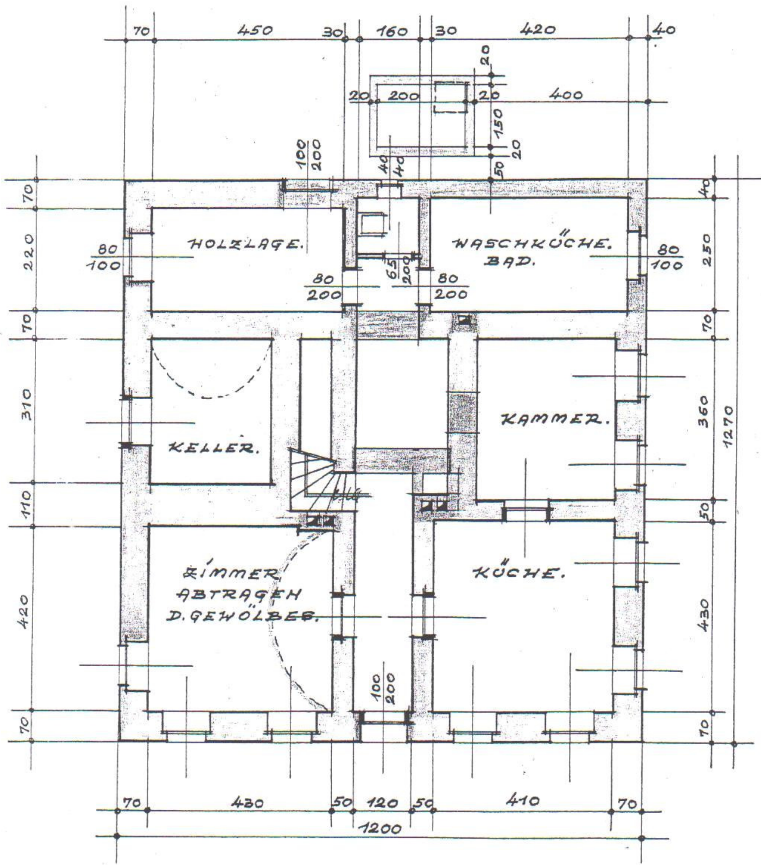
ERDGESCHOSS.
